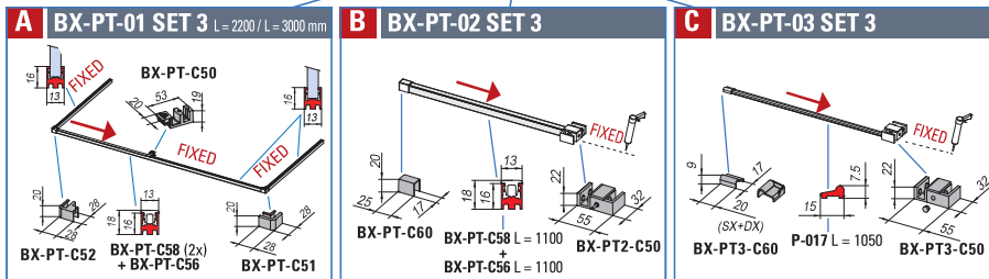
PROFILI A TERRA / FLOOR PROFILES / BODENPROFILE ▶ 106
