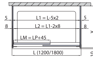
PROFILI A TERRA FLOOR PROFILES - BODENPROFILE ▶ 106 xme632f
