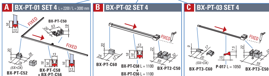
PROFILI A TERRA / FLOOR PROFILES / BODENPROFILE ▶ 106
