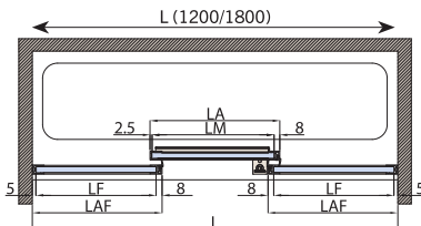
PROFILI A TERRA FLOOR PROFILES - BODENPROFILE ▶ 106
