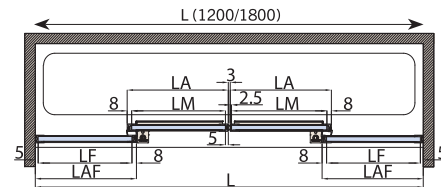
PROFILI A TERRA FLOOR PROFILES - BODENPROFILE ▶ 106
