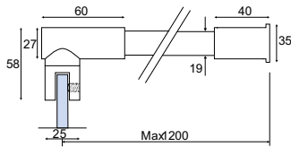
B-161 €► BX.322 • Barra di fissaggio vetro/muro 90°. • Glass to wall 90° fixing bar. • Stabilisationsstange Glas-Wand. CR - NS
