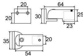
B-164 €► BX.333 • Raccordo a 135° per tubo Ø19 mm. • 135° connector for 19 mm tube Forged brass. • Rohrverbinder 135° für Rohr Ø 19 mm. CR - NS
