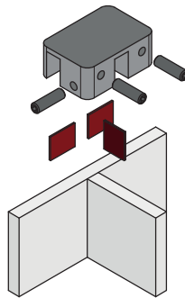
SC-204 • Connettore 4 vie • 4- \square a \square s connector • 4-Wege Verbinder
